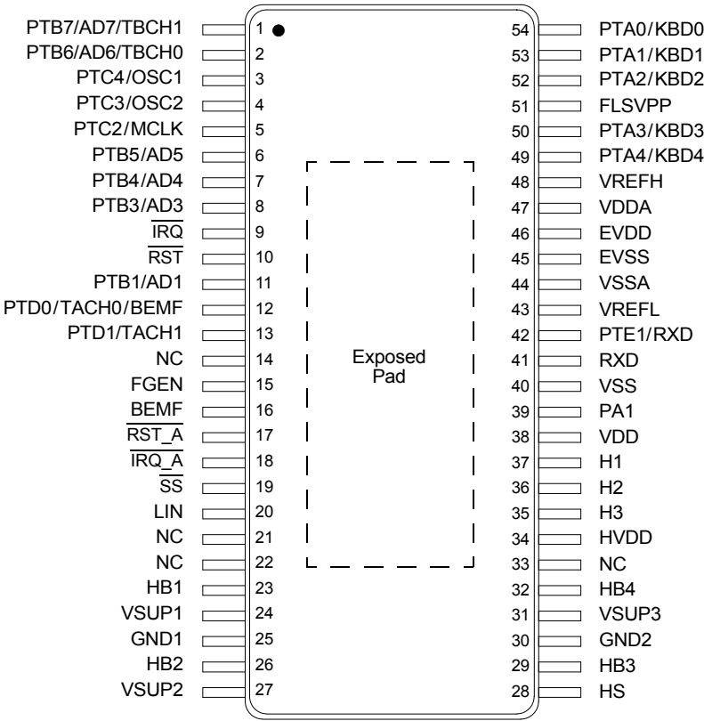
Figure 3. 908E625 Pin Connections (Transparent Package Top View)
