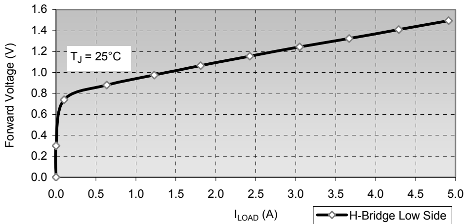
Figure 6. Free Wheel Diode Forward Voltage vs. I_{\text{LOAD}}
