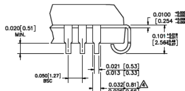
DETAIL "A"
