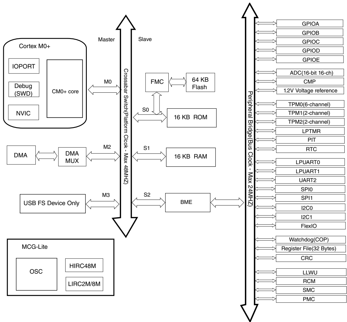
Figure 1. System diagram
