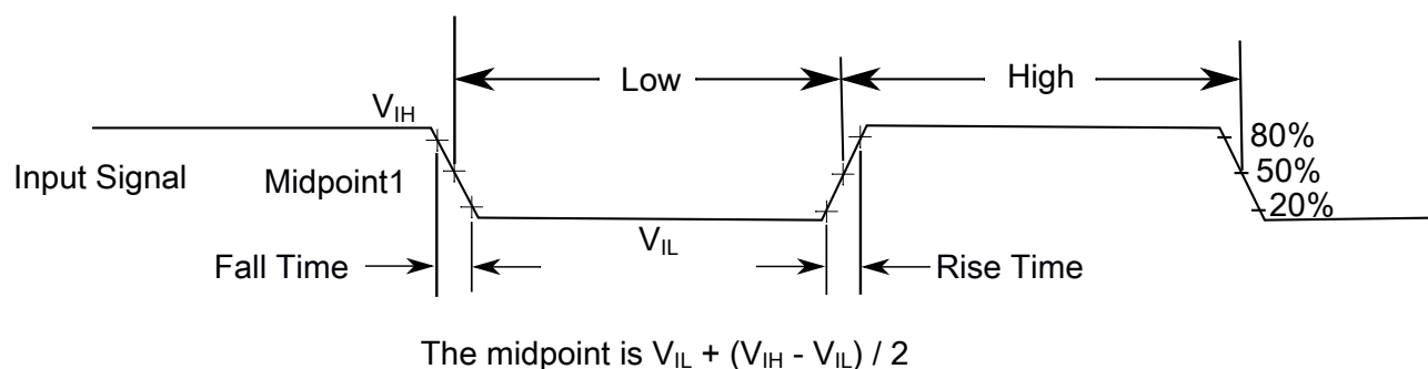
Figure 19. Input signal measurement reference
