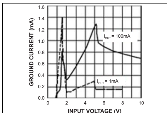
FIGURE 2-5: Ground Current vs. Input Voltage.
