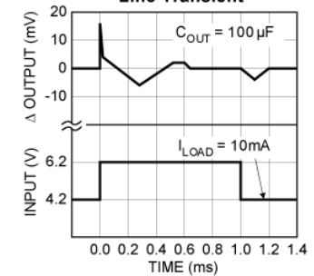
MIC2950x Line Transient
