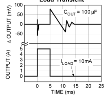
MIC2950x Load Transient
