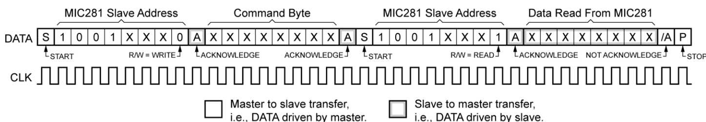
Figure 2. Read_Byte Protocol
