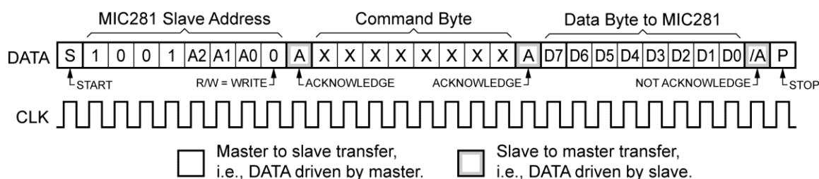
Figure 1. Write_Byte Protocol
