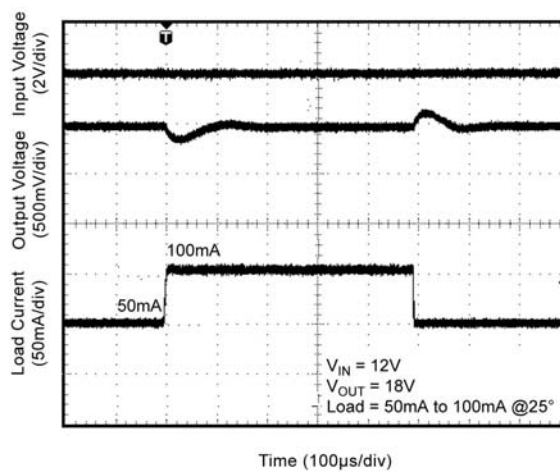
Load Transient
