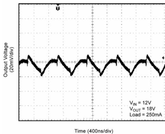
Ripple Waveform
