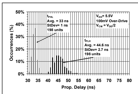
FIGURE 2-24: Low-to-High and High-to-Low Propagation Delays.
