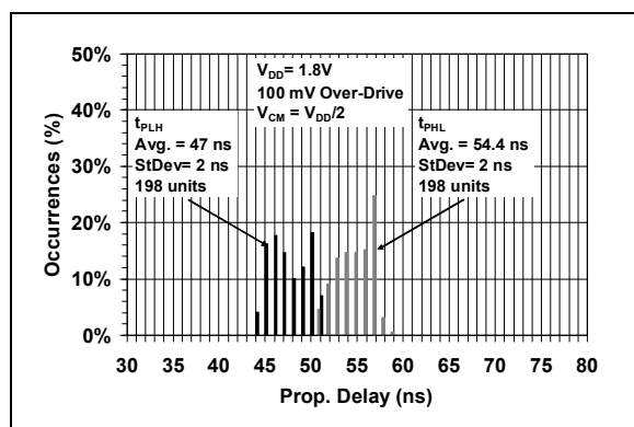
FIGURE 2-21: Low-to-High and High-to-Low Propagation Delays.
