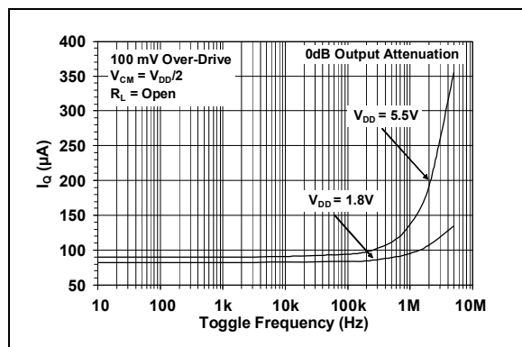
FIGURE 2-19: Quiescent Current vs. Toggle Frequency.
