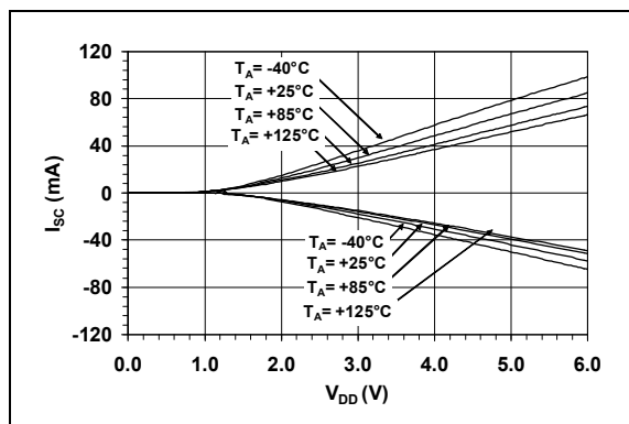
FIGURE 2-22: Short-Circuit Current vs. Supply Voltage vs. Temperature.
