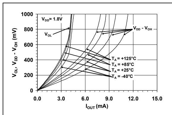
FIGURE 2-20: Output Headroom vs. Output Current.
