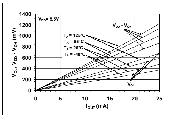
FIGURE 2-23: Output Headroom vs. Output Current.
