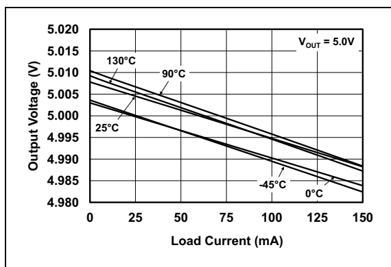
FIGURE 2-12: Output Voltage vs. Load Current.
