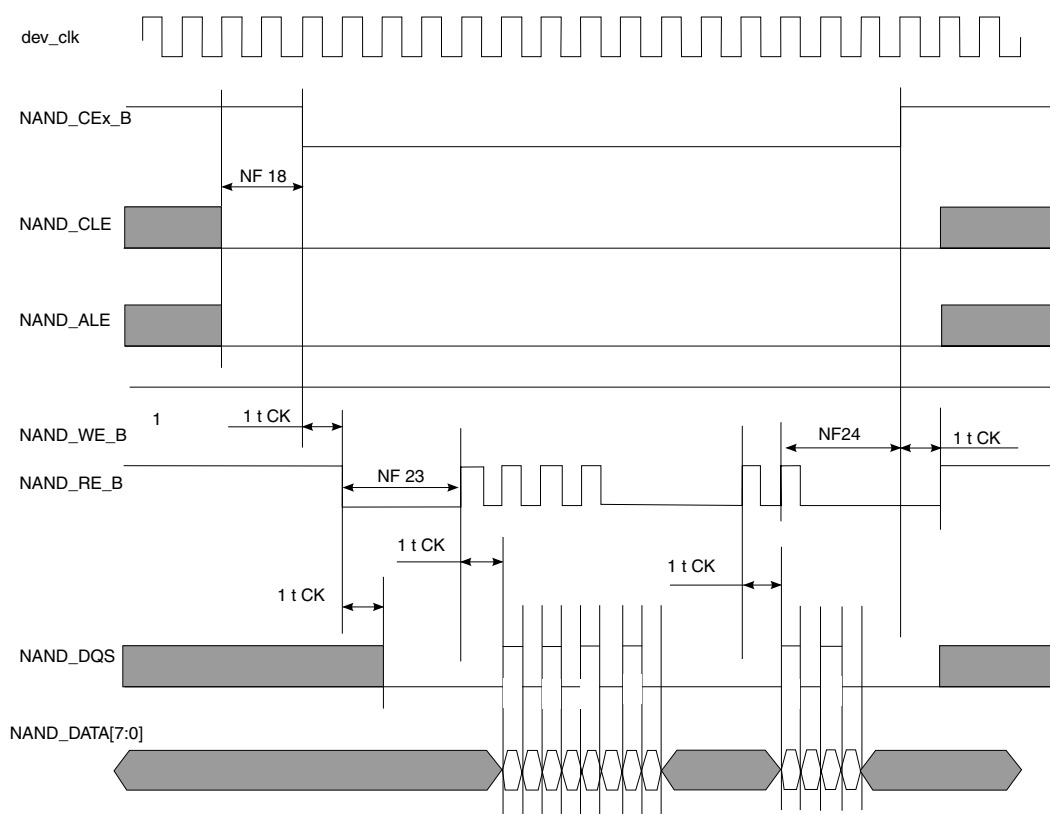
Figure 33. Samsung Toggle Mode Data Read Timing
