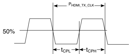
Figure 52. TMD5 Clock Signal Definitions
