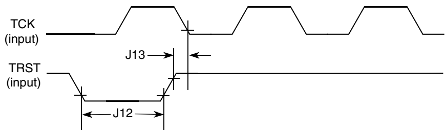
Figure 25. TRST Timing Diagram
