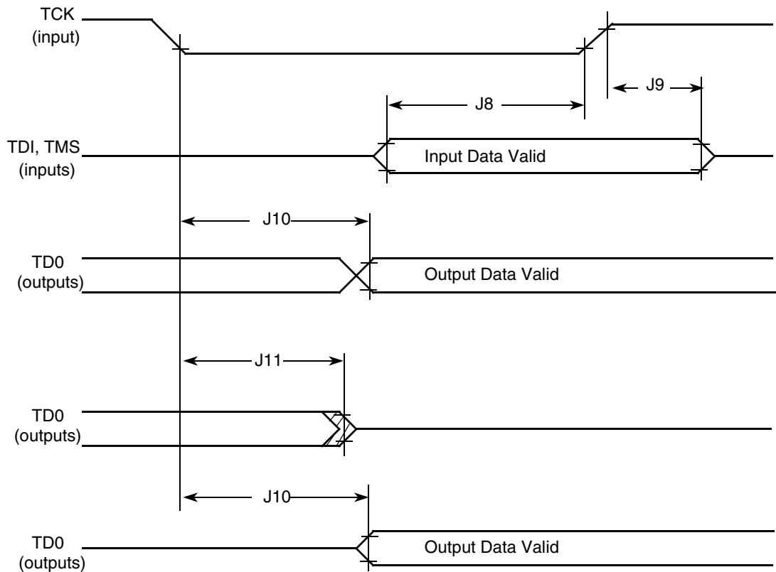
Figure 24. Test Access Port (TAP) Diagram
