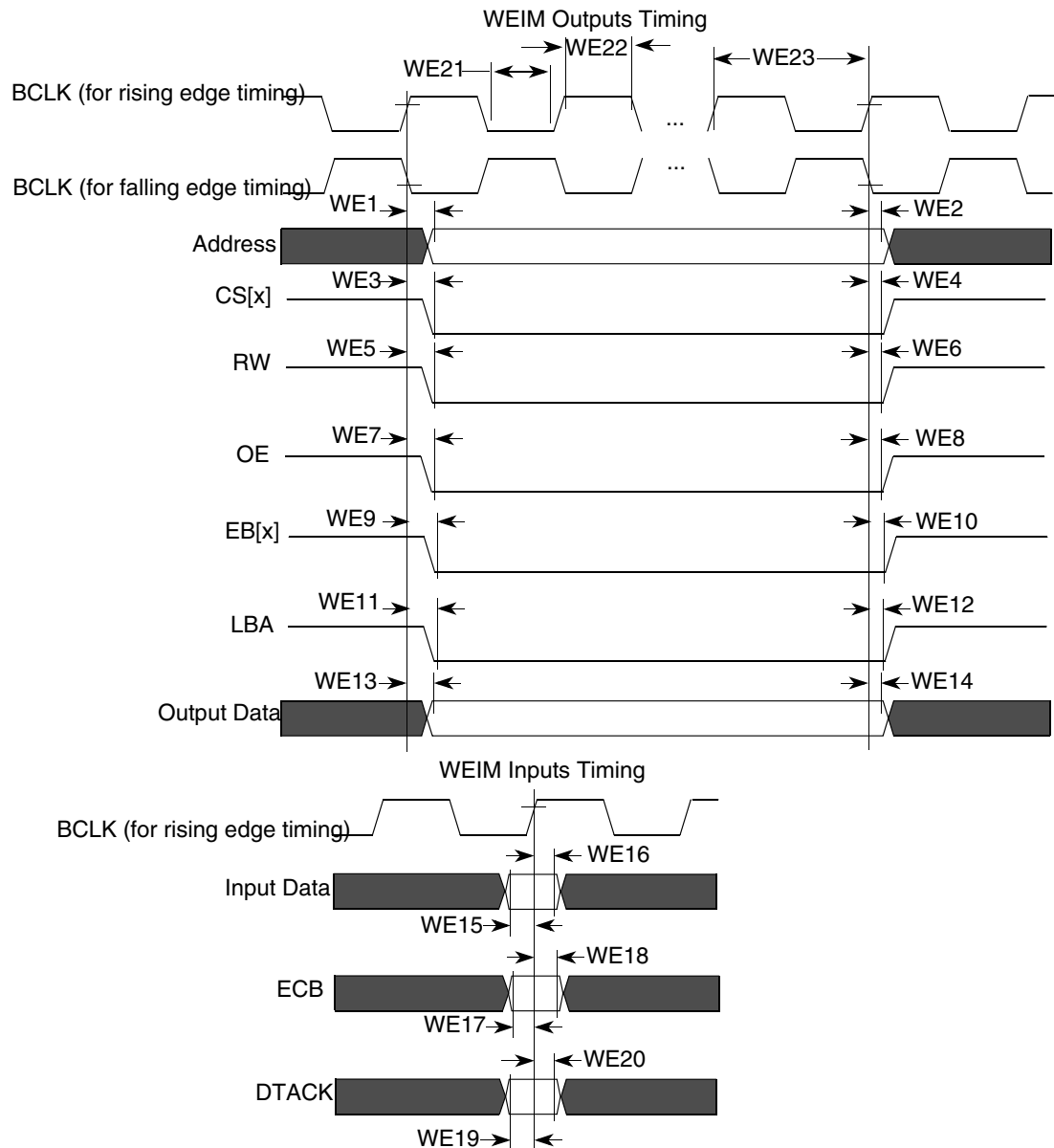
Figure 53. WEIM Bus Timing Diagram
