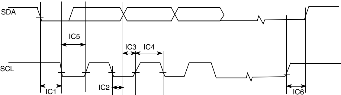
Figure 21. I²C Bus Timing Diagram
