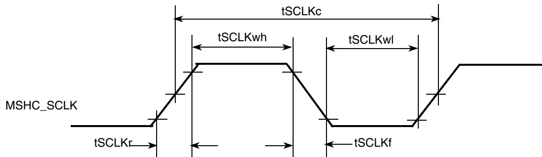
Figure 30. MSHC_CLK Timing Diagram
