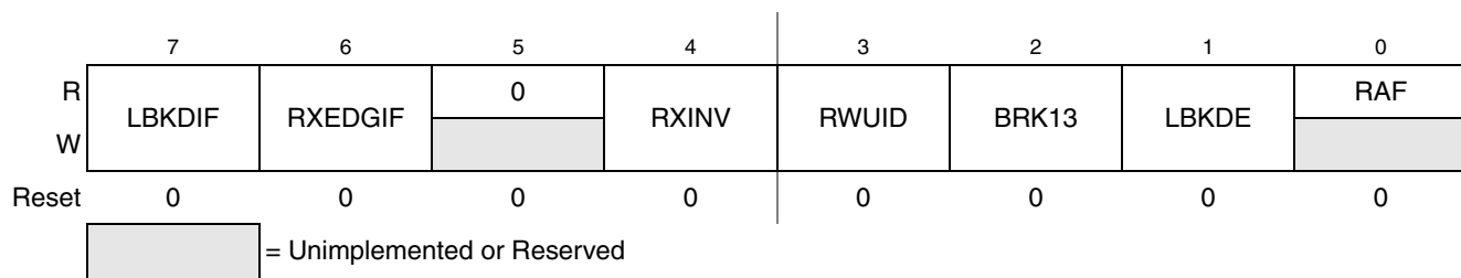
Figure 14-9. SCI Status Register 2 (SCIS2)
