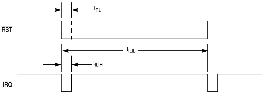
Figure 18-6. \overline{RST} and \overline{IRQ} Timing
