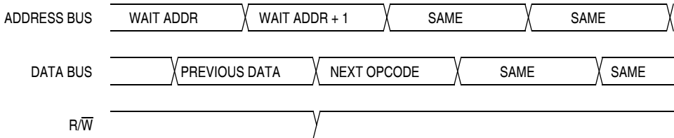
Figure 14-14. Wait Mode Entry Timing
