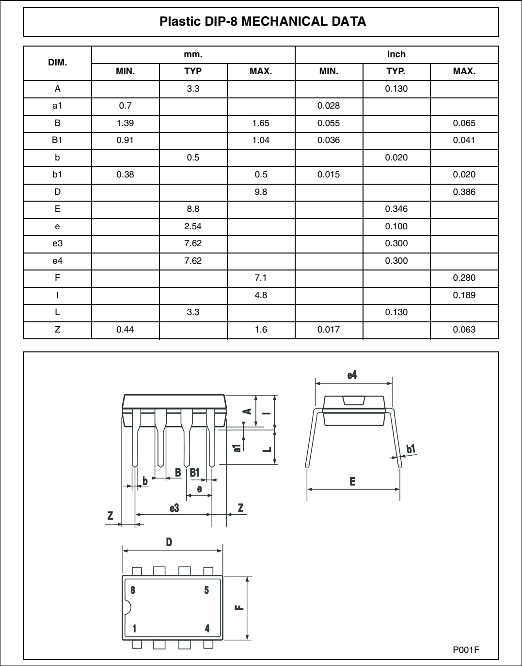
Figure 8. DIP8 package
