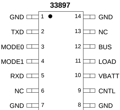
Figure 3. 33897 Pin Connections
