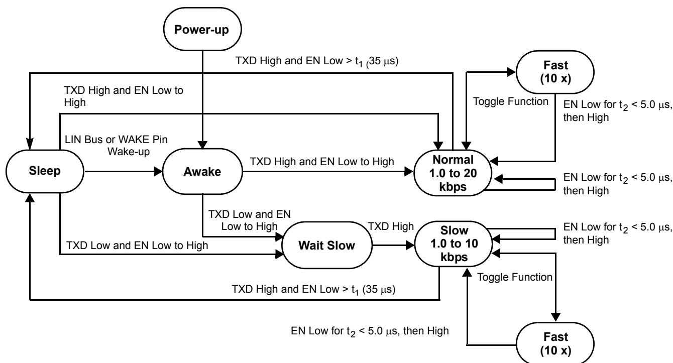
Figure 15. Operational and Transitional Modes State Diagram
