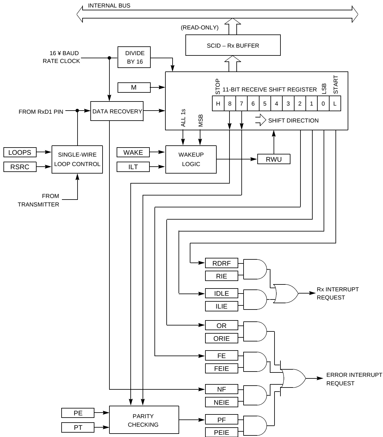
Figure 23. SCI Receiver
