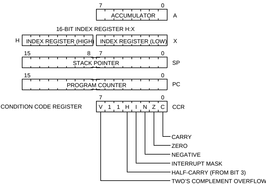
Figure 18. CPU Registers
