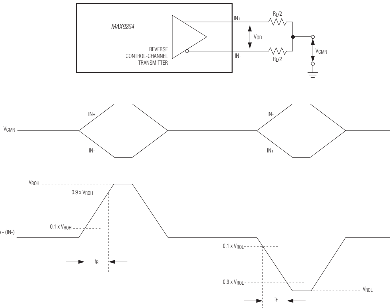
Figure 13. Reverse Control-Channel Output Parameters
