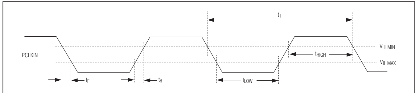
Figure 5. Serializer Parallel Input Clock Requirements
