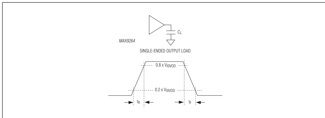
Figure 17. Deserializer Output Rise and Fall Times
