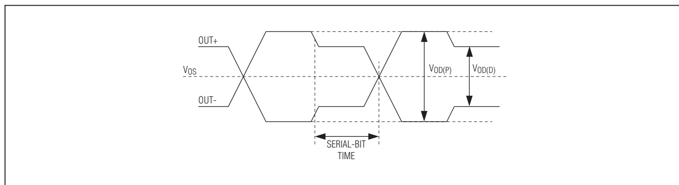
Figure 2. Serializer Output Waveforms at OUT+ , OUT-
