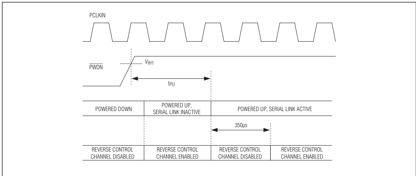
Figure 11. Serializer Power-Up Delay
