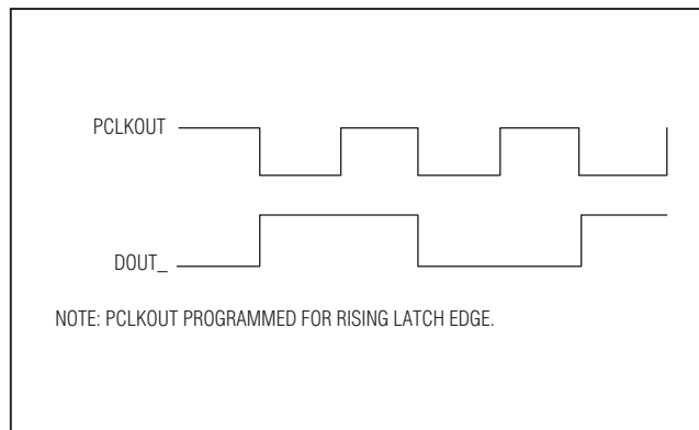
Figure 15. Deserializer Worst-Case Pattern Output
