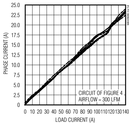
CURRENT-SHARING ACCURACY
