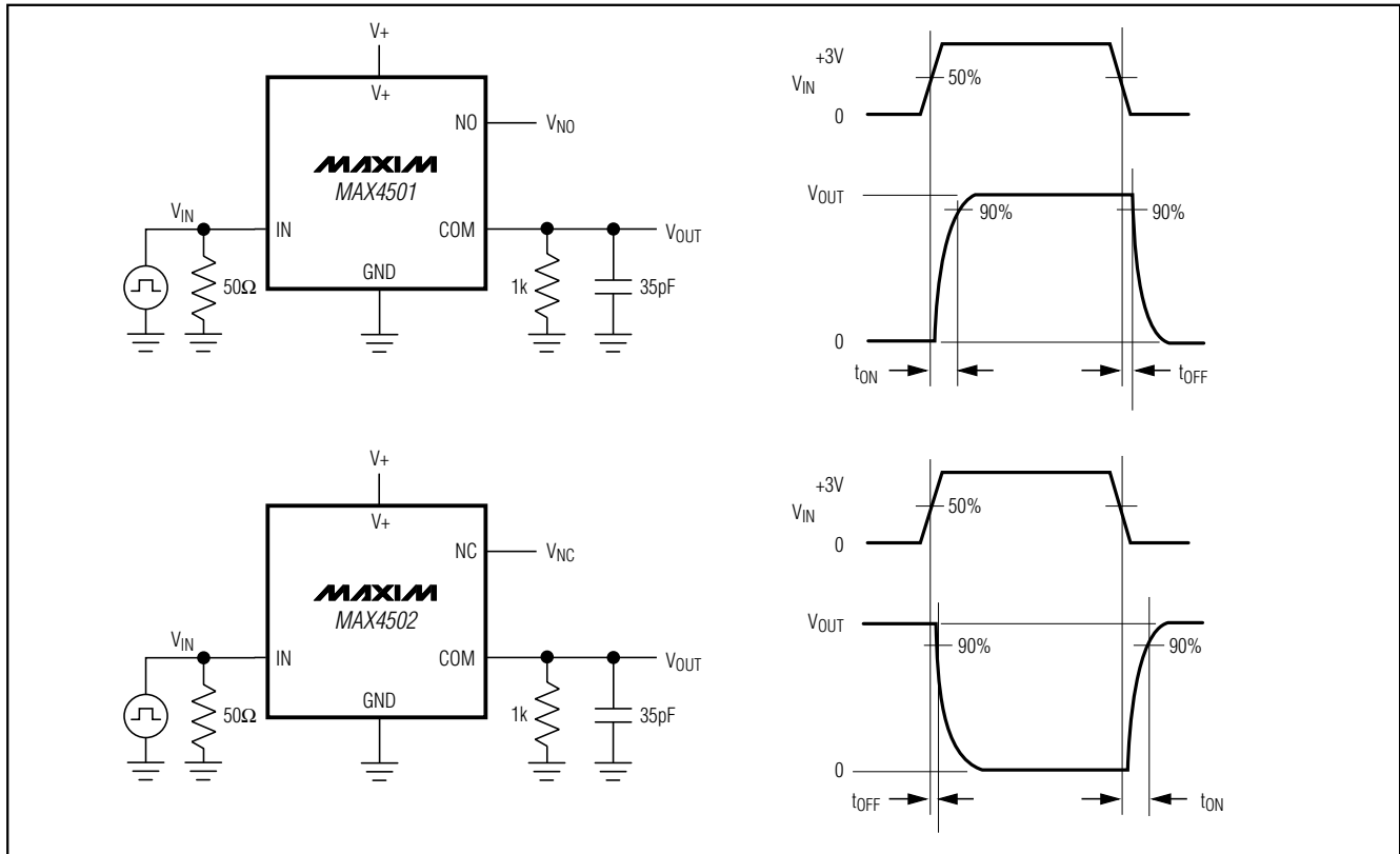
Figure 1. Switching Times
