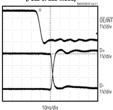
DRIVER ENABLE DELAY (FULL-SPEED MODE)
