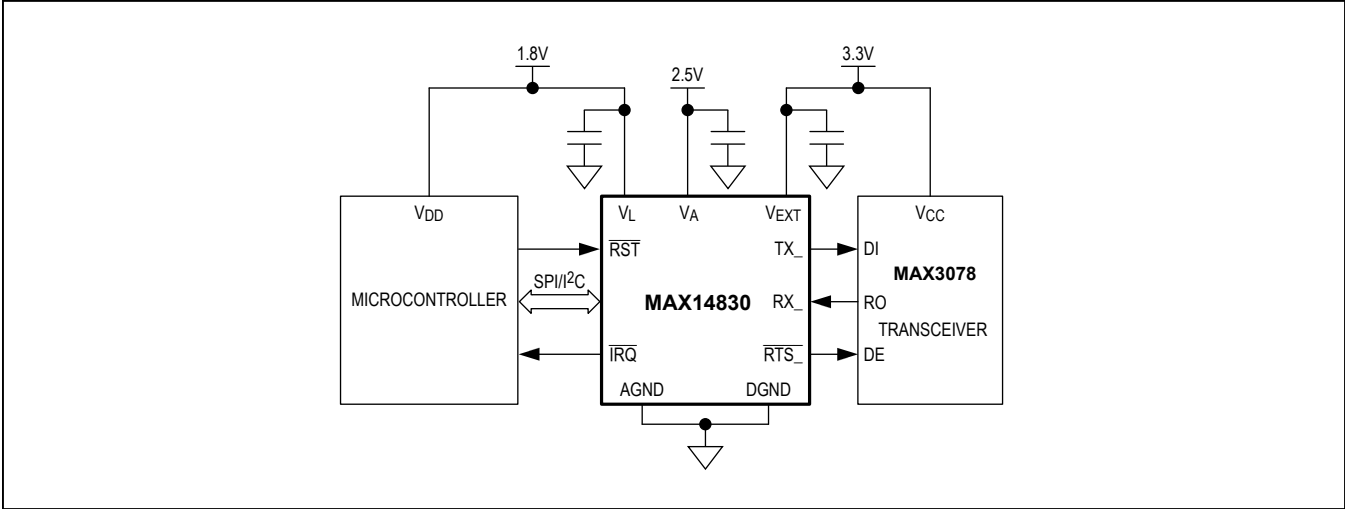
Figure 28. Logic-Level Translation
