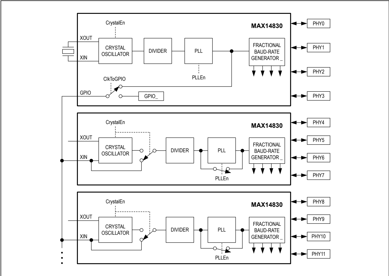
Figure 29. Interchip Synchronization
