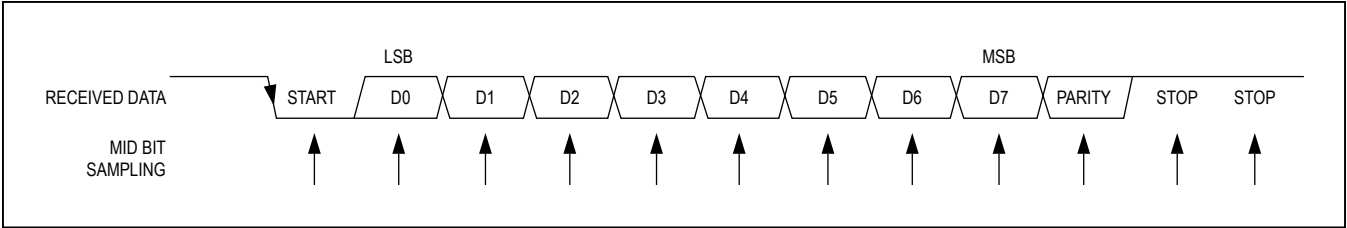
Figure 4. Receive Data Format
