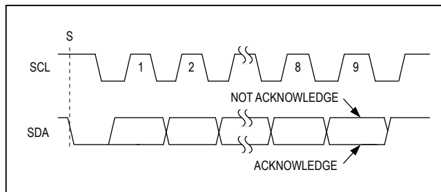
Figure 26. Acknowledge Bits
