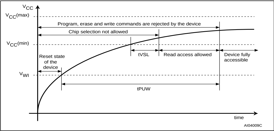
Figure 18. Power-up timing
