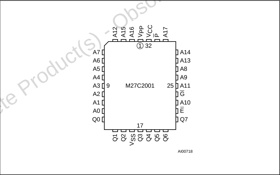
Figure 3. LCC Connections
