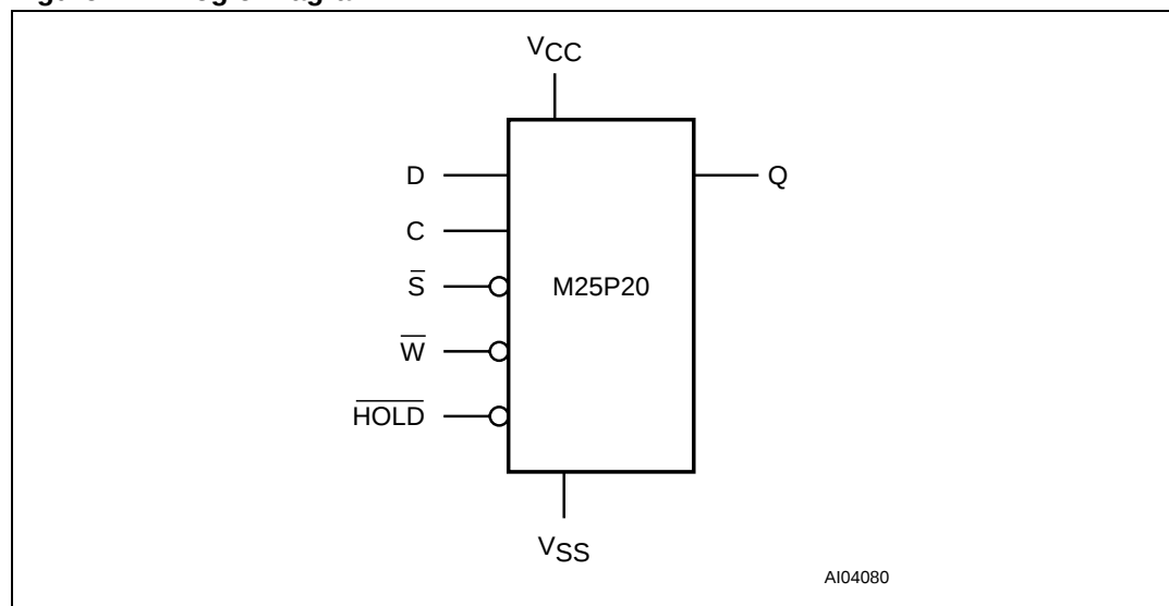
Figure 1. Logic Diagram
