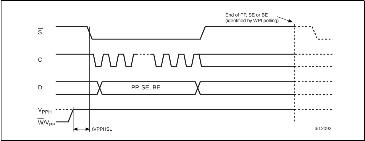
Figure 24. V_{PPH} timing
