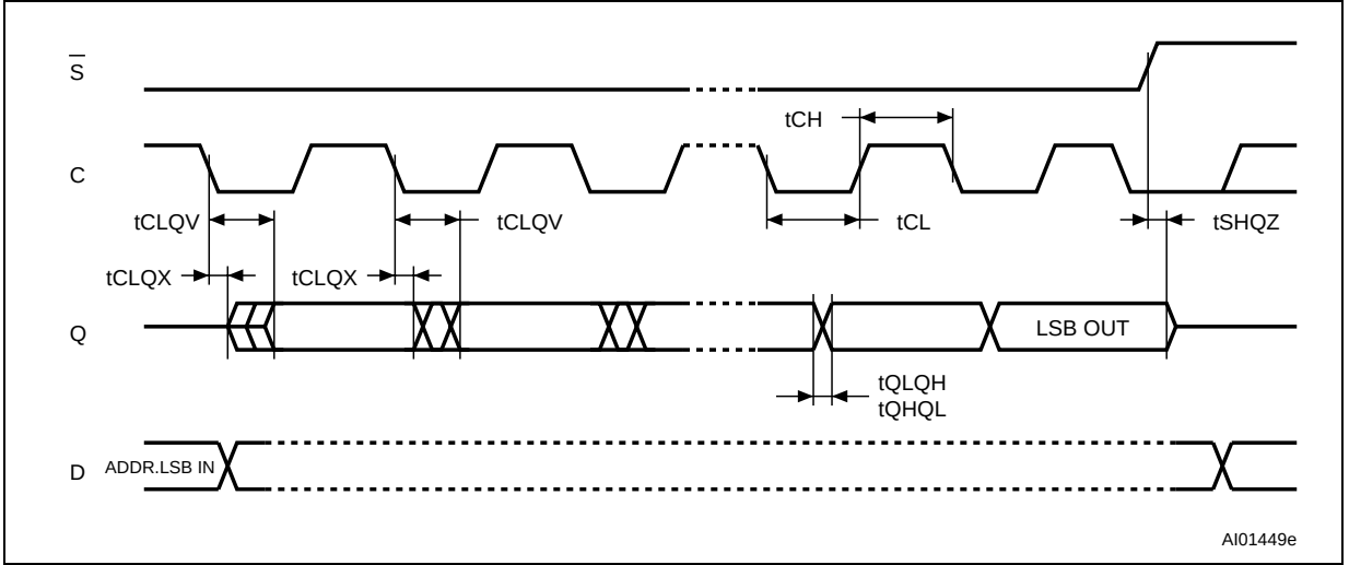
Figure 23. Output timing
