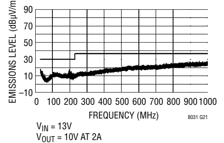
Radiated Emissions
