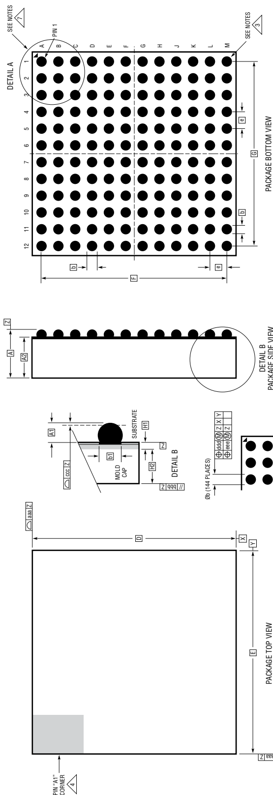
BGA Package 144-Lead (16mm × 16mm × 5.01mm) (Reference LTC DWG # 05-08-1920 Rev C)
