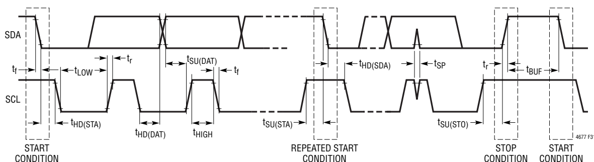
Figure 31. Timing Diagram
