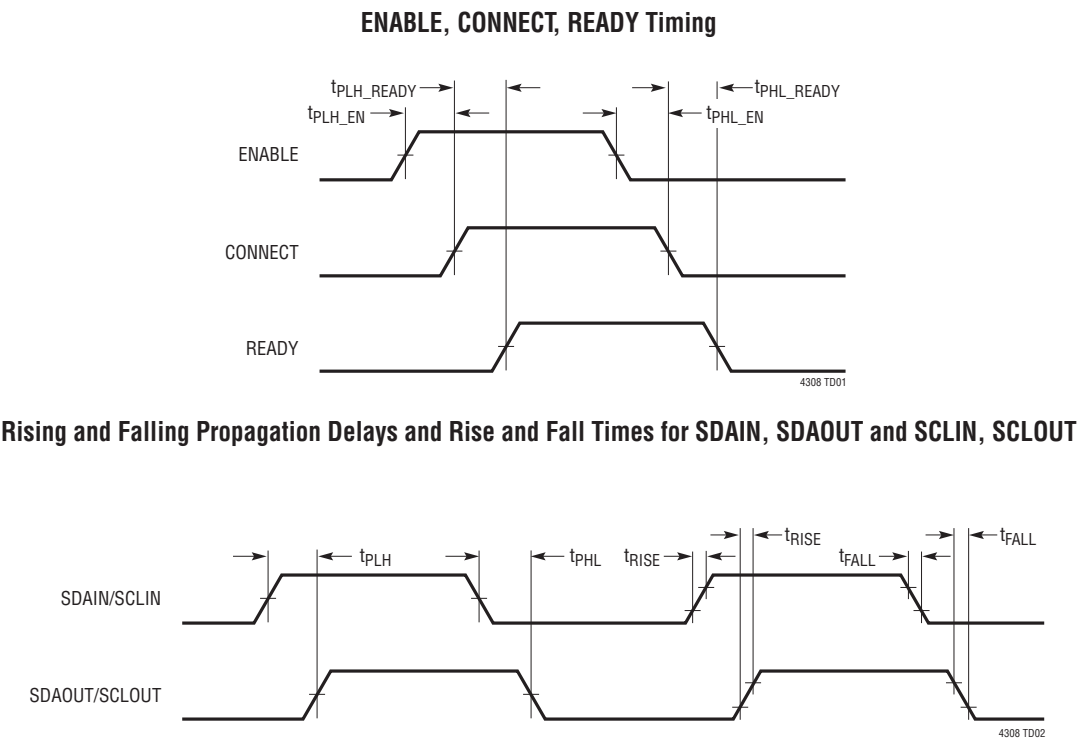
Figure 1. Timing Diagrams
