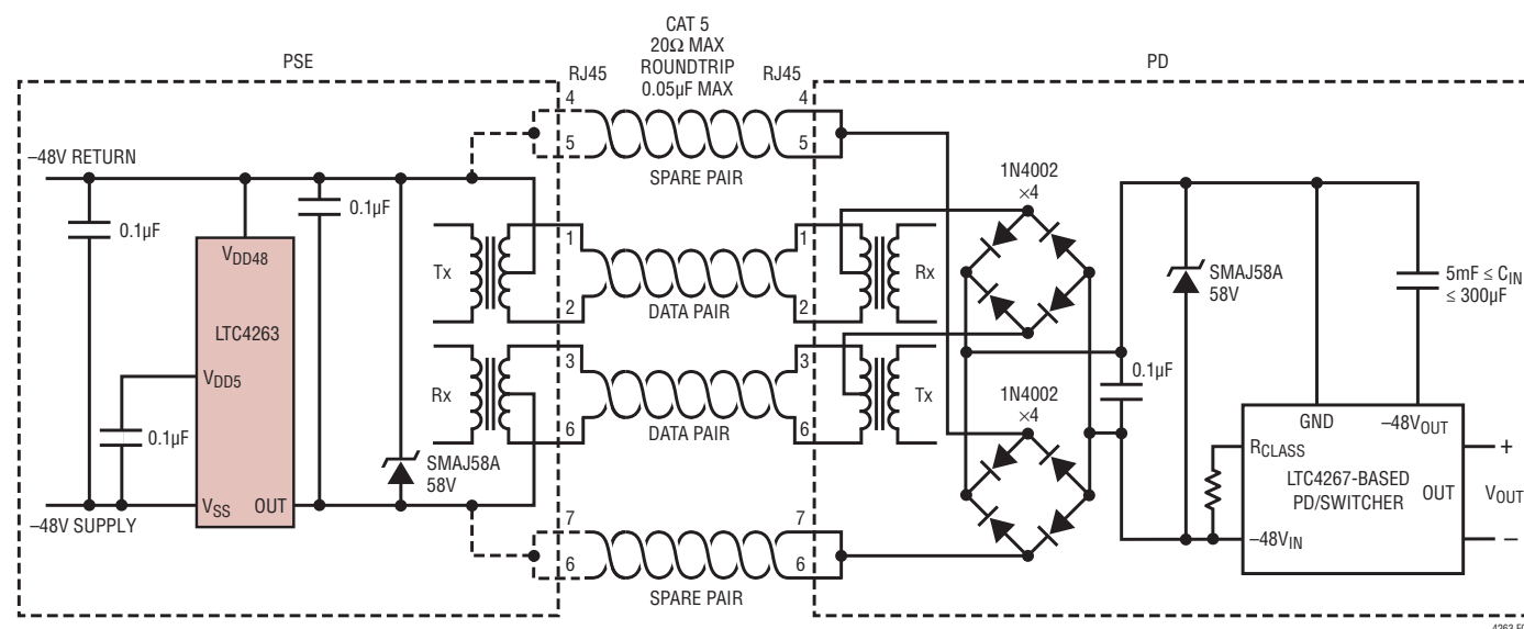
Figure 1. System Diagram
