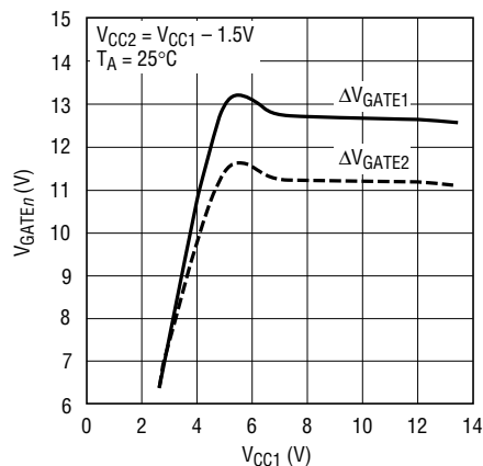
\Delta V_{GATEn} (V_{GATEn} - V_{CC1}) vs V_{CC1}
