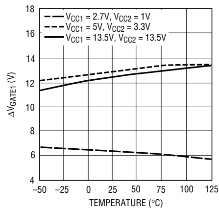
\Delta V_{GATE1} (V_{GATE1} - V_{CC1}) vs Temperature
