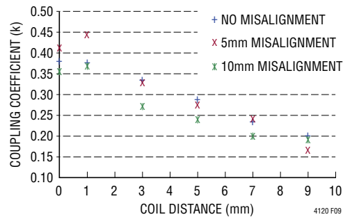
Figure 9. Coupling Coefficient k vs Distance
