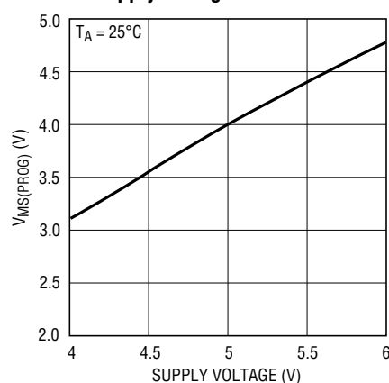
PROG Pin Shutdown Voltage Threshold vs Supply Voltage
