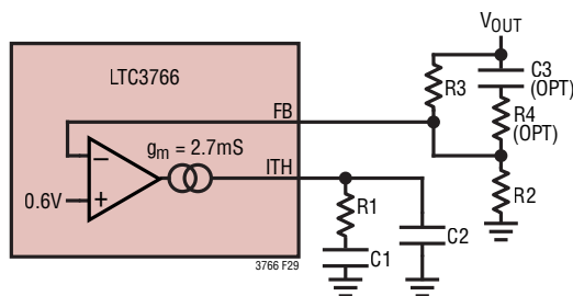
Figure 29. ITH Compensation Network
