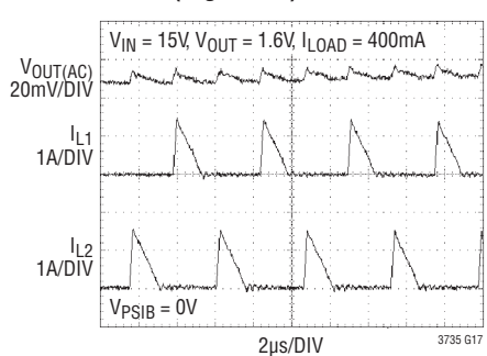
Constant Frequency Low Current Mode (Figure 14)
