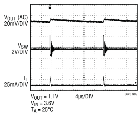
Switching Waveforms at 250μA Load, FMIN/MODE = 0V
