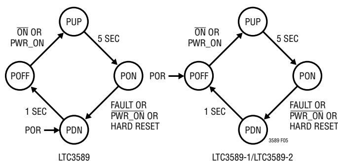
Figure 5. Pushbutton Controller State Diagram
