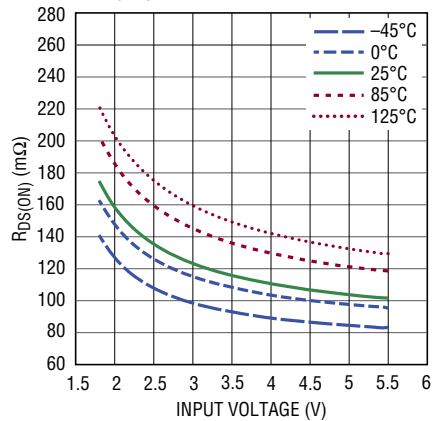
R_{DS(ON)} for P-Channel Switch A
