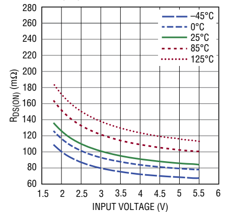
R_{DS(ON)} for N-Channel Switch C
