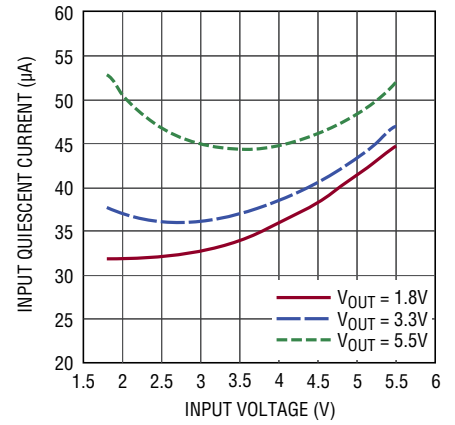
No-Load Quiescent Current in Burst Mode Operation (MODE = V_{IN} )
