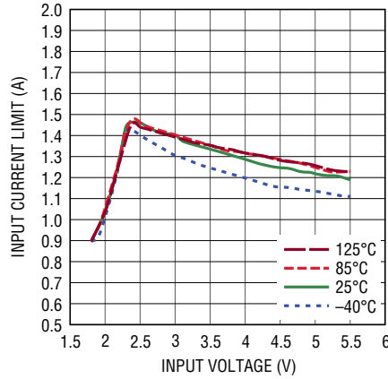
Input Current Limit vs Supply Voltage, V_{OUT} = \text{GND}
