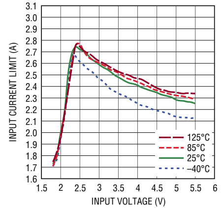
Input Current Limit vs Supply Voltage, V_{OUT} = 3.3\text{V}
