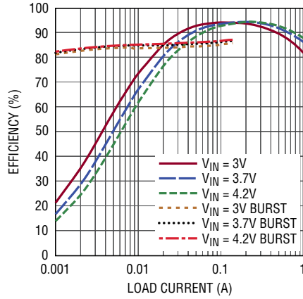
Efficiency Li-Ion (3V, 3.7V, 4.2V) to 3.3V Output
