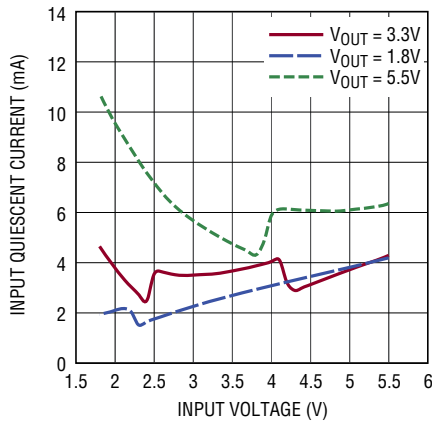
No-Load Quiescent Current in PWM Mode Operation
