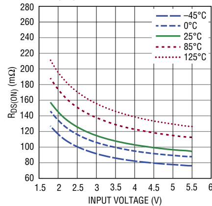
R_{DS(ON)} for N-Channel Switch B
