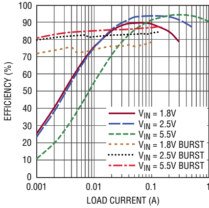
Efficiency 3.3V vs Load Current
