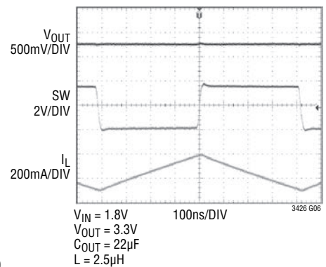
Switching Waveforms
