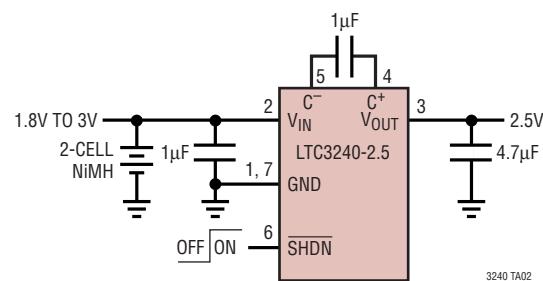
2.5V Output from 2-Cell NiMH
