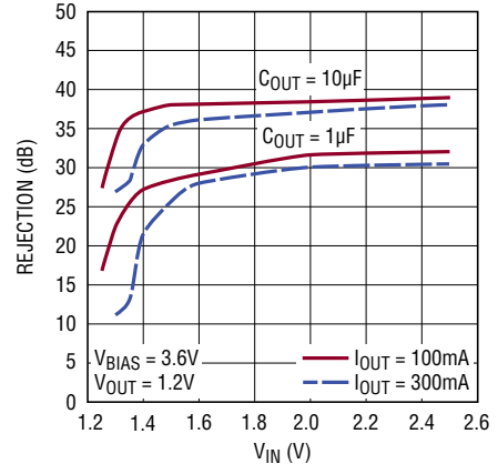
3MHz V_{IN} Supply Rejection
