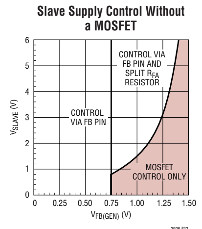
Figure 22. Regions of Possible Slave Control Without a MOSFET
