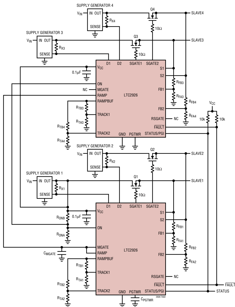
Chaining to Track/Sequence More Supplies
