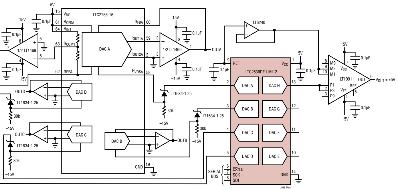
LTC2636 DACs Adjust LTC2755-16 Offsets, Amplified with LT1991 PGA to ±5V
