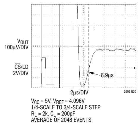
Settling to \pm 1\text{LSB}
