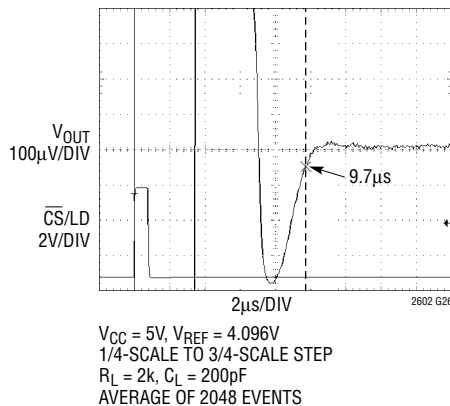
Settling to \pm 1\text{LSB}
