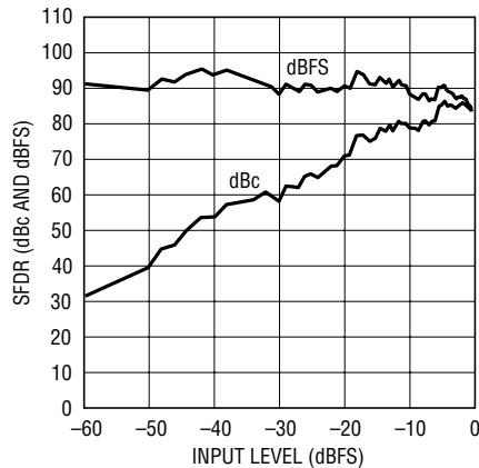
LTC2252: SFDR vs Input Level, f_{IN} = 70\text{MHz} , 2V Range, 105Mps
