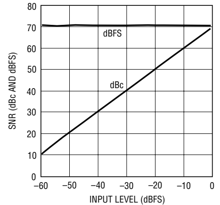
LTC2252: SNR vs Input Level, f_{IN} = 70\text{MHz} , 2V Range, 105Mps
