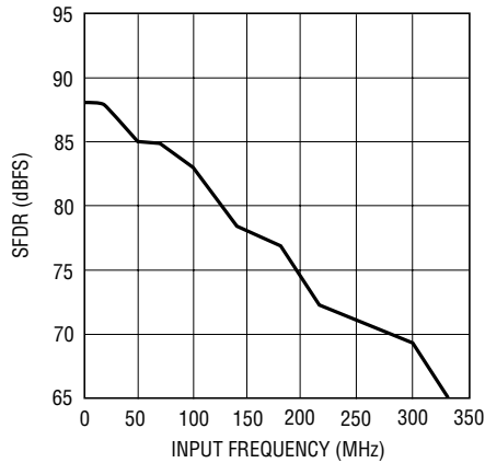
LTC2252: SFDR vs Input Frequency, -1dB, 2V Range, 105Mps
