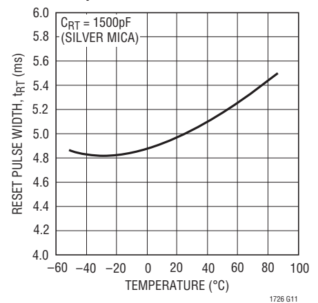
Reset Pulse Width vs Temperature
