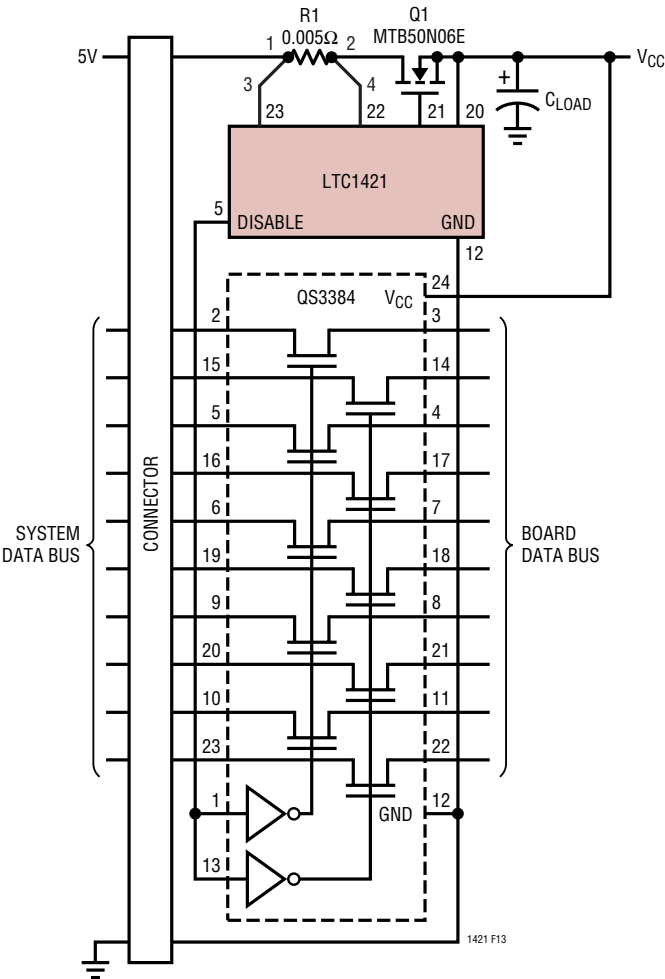
Figure 13: Buffering the Data Bus
