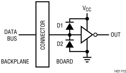
Figure 12. Typical Logic Gate Loading the Data Bus
