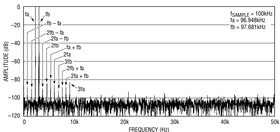
Figure 5. Intermodulation Distortion
