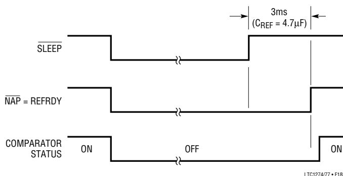
Figure 18b. Power Saved in Sleep Mode ( \overline{NAP} = \text{REFRDY} )
