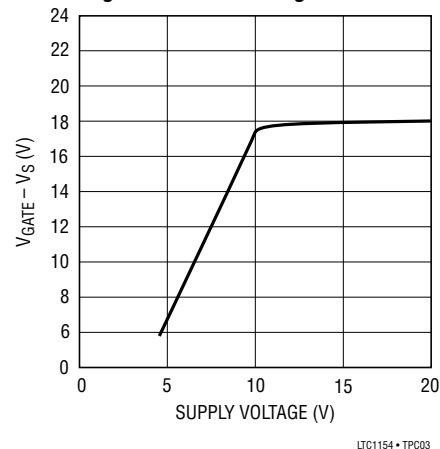
High Side Gate Voltage
