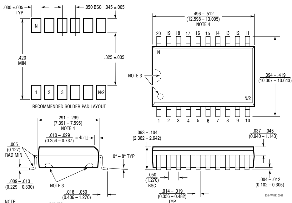
SW Package 20-Lead Plastic Small Outline (Wide .300 Inch) (Reference LTC DWG # 05-08-1620)
